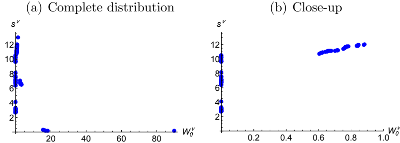
Figure 1: Skills versus wealth for typical simulation
