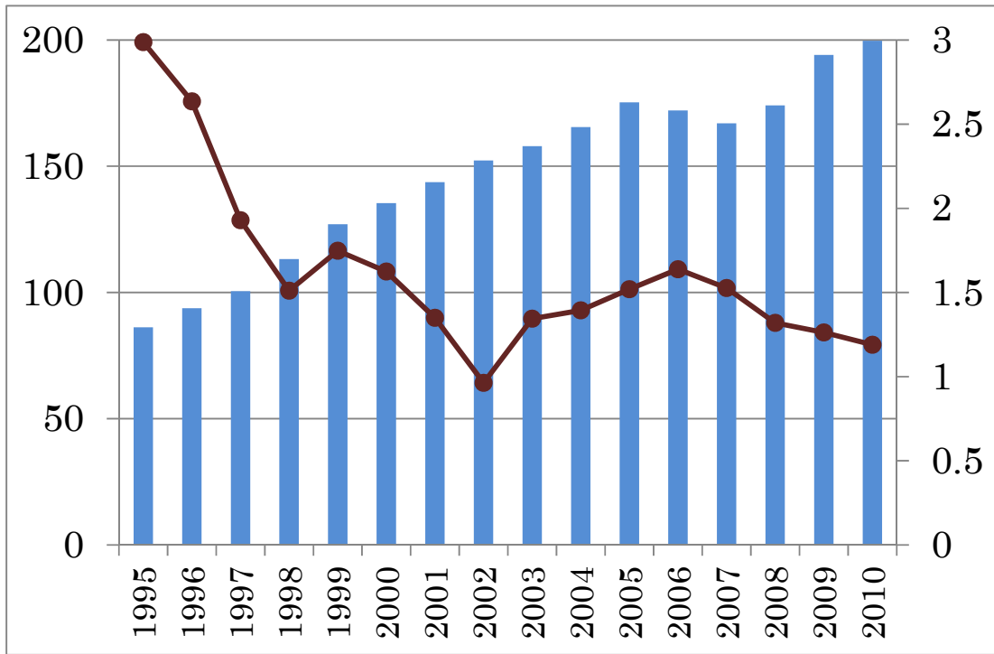
Figure 1 Debt/GDP ratio and JGB yield: 1995–2010
