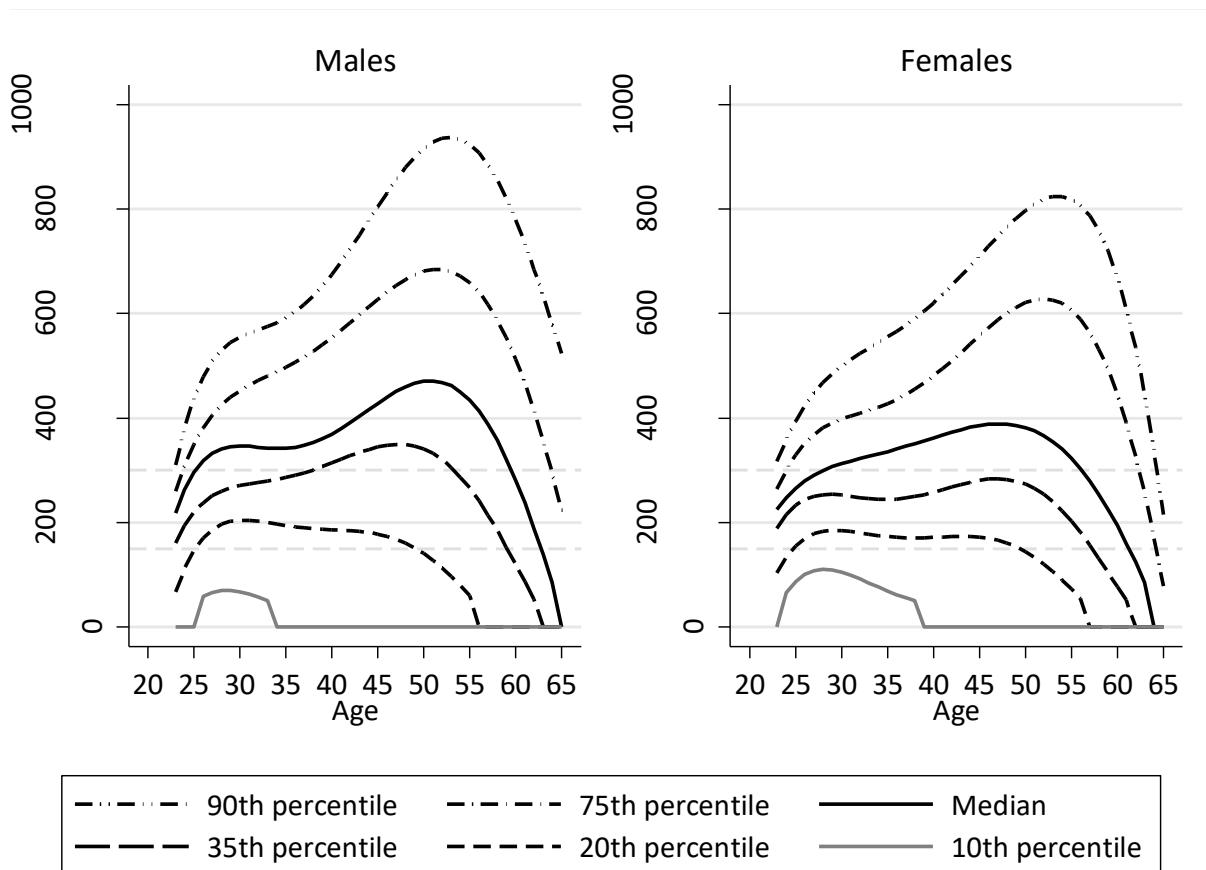
Figure 6: Quantile estimates of single BA graduate earnings: LFS data
